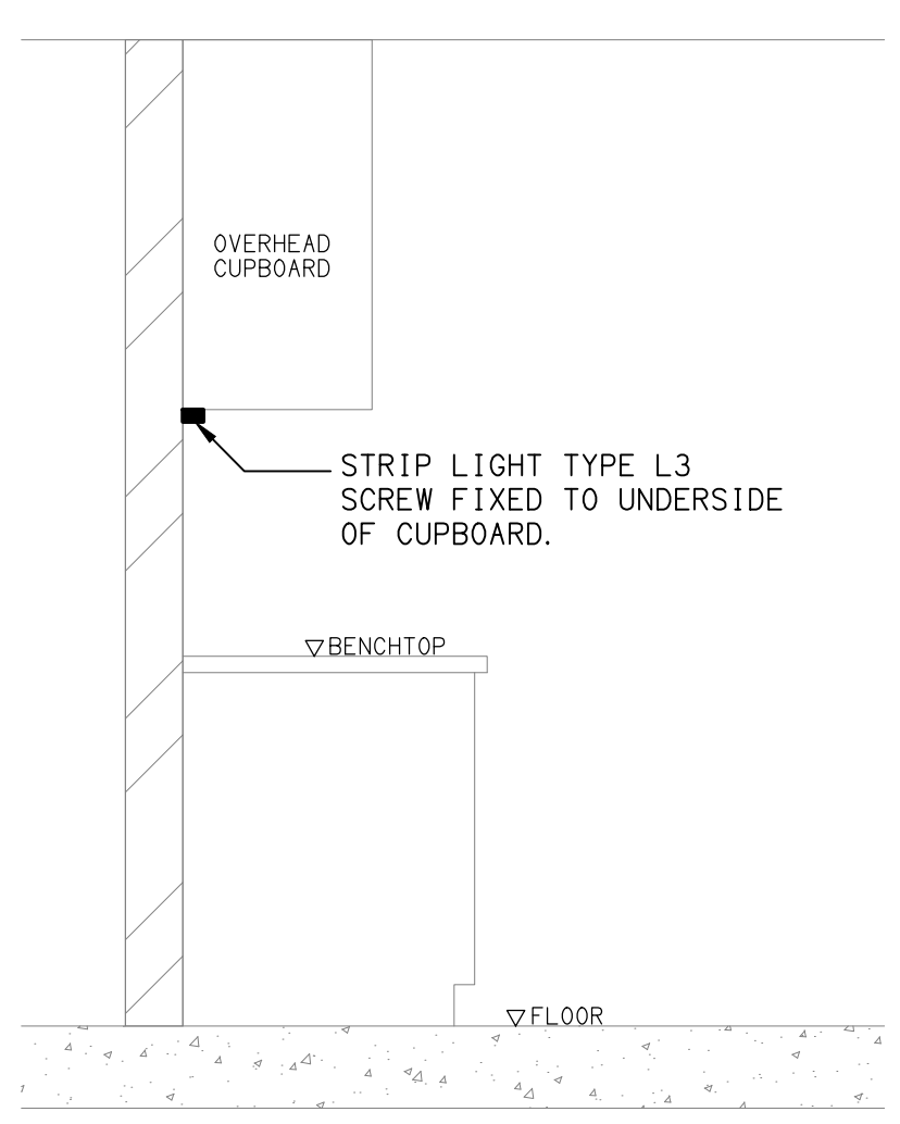
DETAIL STRIP LIGHT TYPE "L3" MOUNTING NOT TO SCALE
